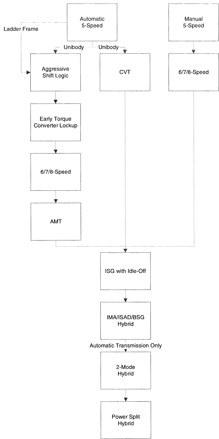
Figure V-3. Transmission Technology Decision Tree
