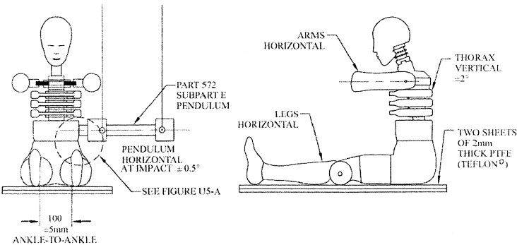
Figure U5 ABDOMEN IMPACT
