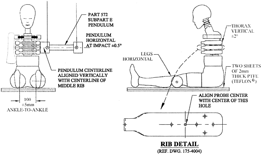
Figure U4 THORAX IMPACT
