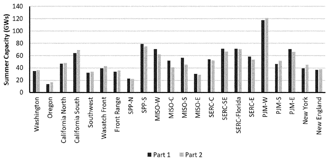
Figure D.3: Comparison of Capacity by TPR, Part 1 vs. Part 2 (2024) 151
