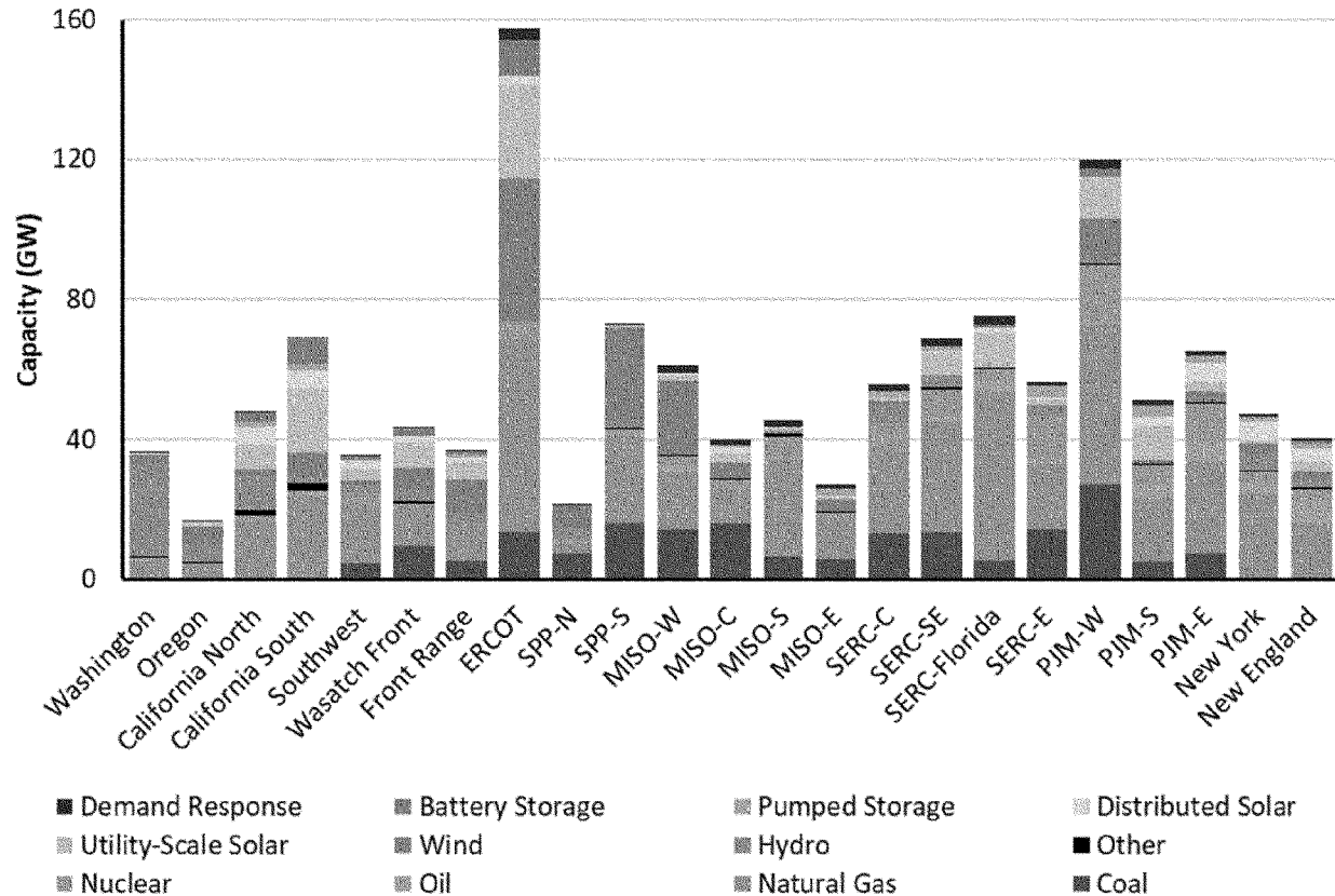
Figure 5.2: Capacity, Existing + Tier 1 Resources (2024 Case)
