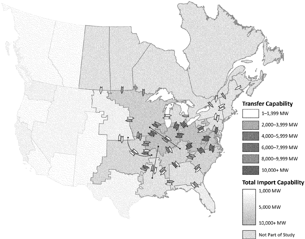
Figure 4.7: Transfer Capabilities of Eastern Interconnection Interfaces (Summer)
