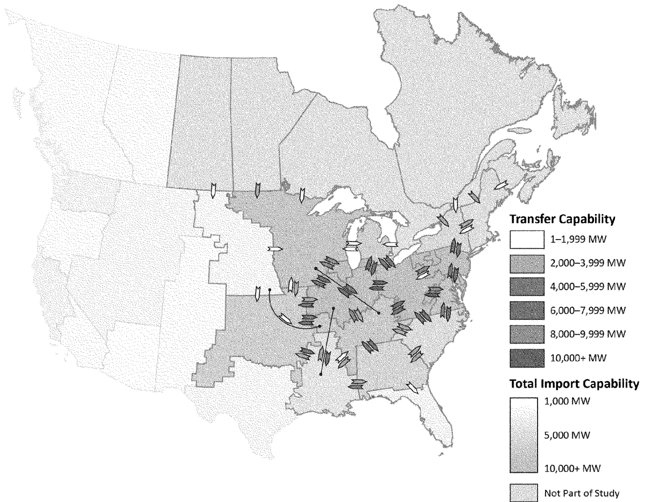
Figure 4.8: Transfer Capabilities of Eastern Interconnection Interfaces (Winter)
