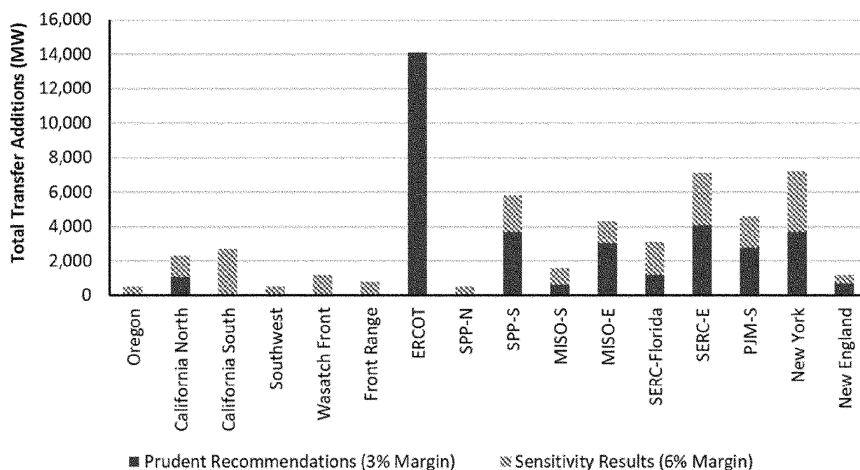
Figure 8.1: Change to Transfer Capability Additions
