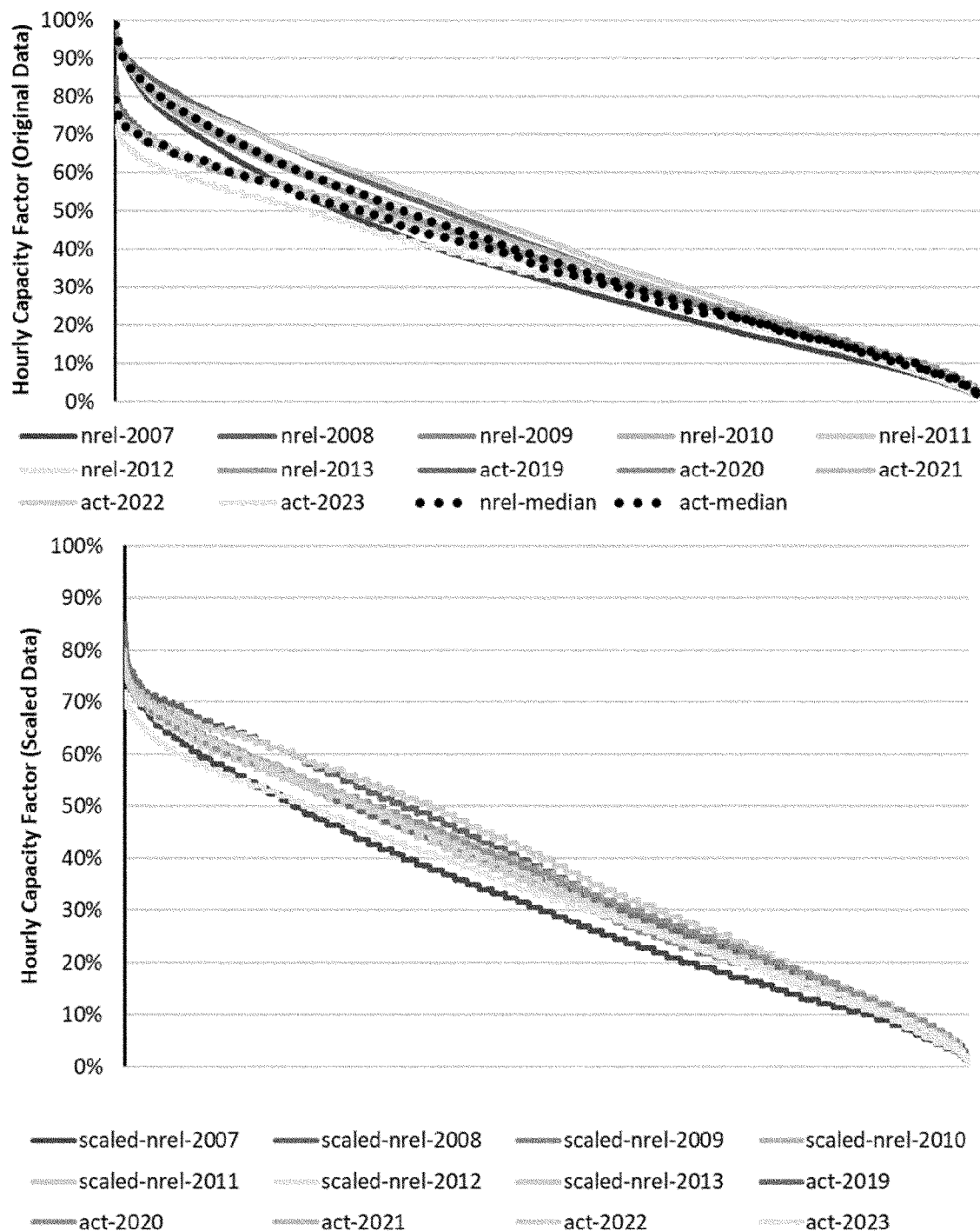
Figure F.1: Example of Scaling Synthetic Weather Data to Align with Historical Actual Data (ERCOT Land-Based Wind)
