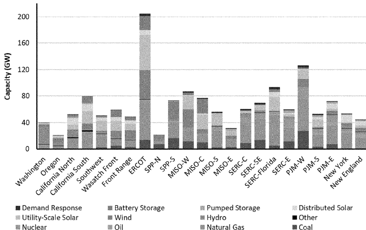
Figure 5.3: Capacity, Existing + Tier 1 + Replace Retirements (2033 Case)
