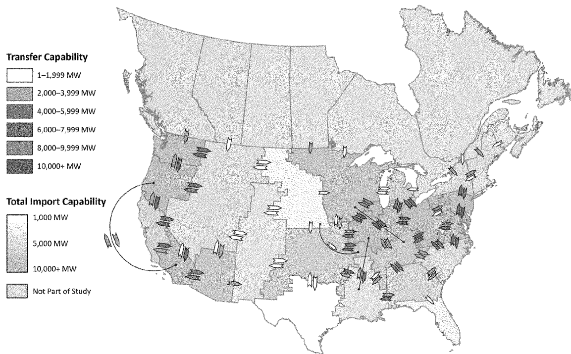
Figure ES.3: Transfer Capabilities (Winter)
