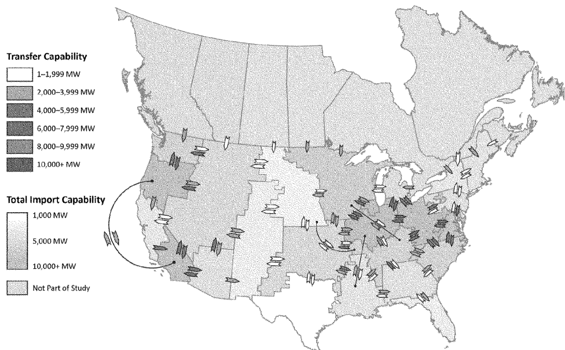
Figure ES.2: Transfer Capabilities (Summer)
