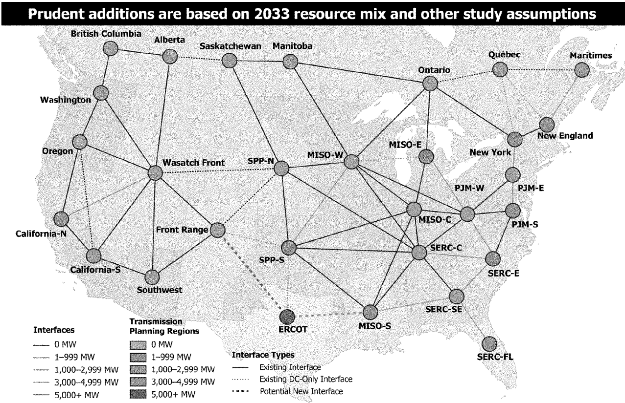
Figure ES.5: Prudent Additions to Transfer Capability
