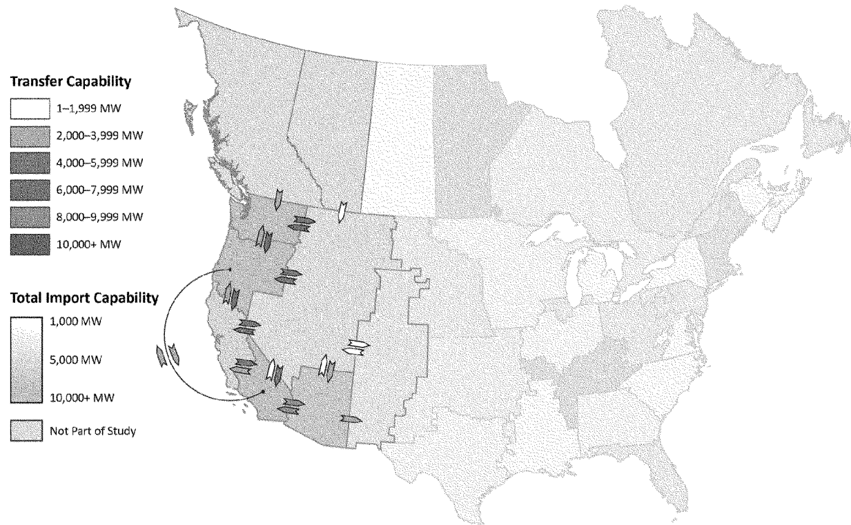
Figure 4.2: Transfer Capabilities for Western Interconnection Interfaces (Winter)
