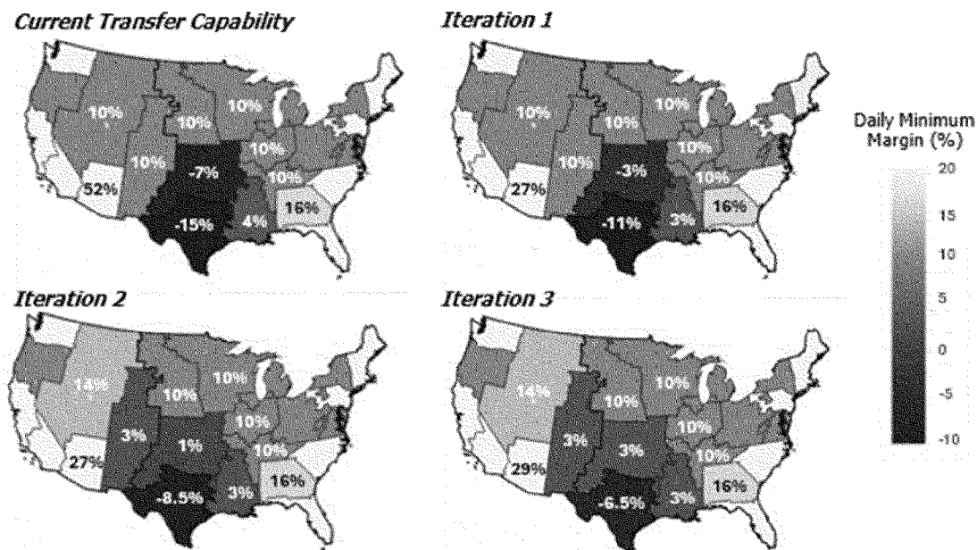
Figure 7.3: Resource Saturation Around ERCOT, February 16, WY2021 (2033 Case)
