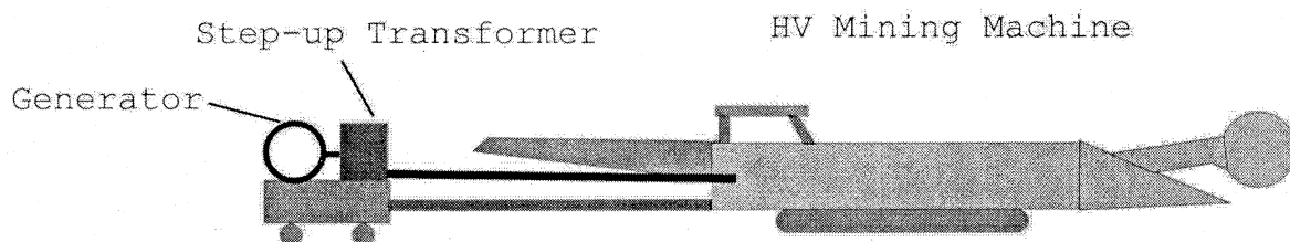
Figure 4-Power Source-75.829(c) (3) Generator Supplies 480/995 volts to step-up transformer for 2300 volts for tramming
