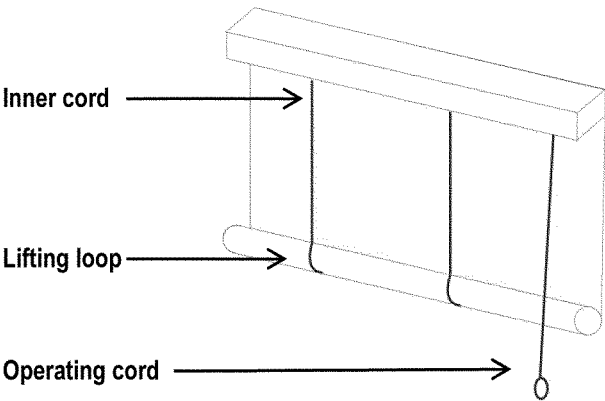
Figure 5. Roll-up blind
