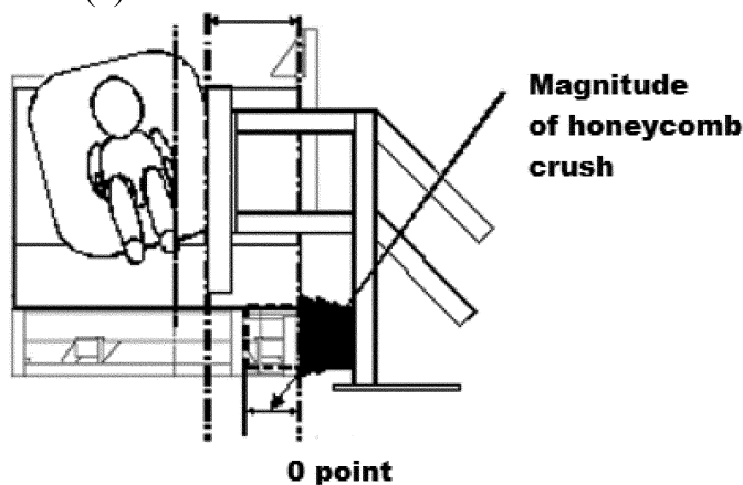
Figure 3 - Takata Side Impact Sled System--(a) Pre-test condition, (b) at time of door contact with CRS, and (c) at end of test (final travel of door).
