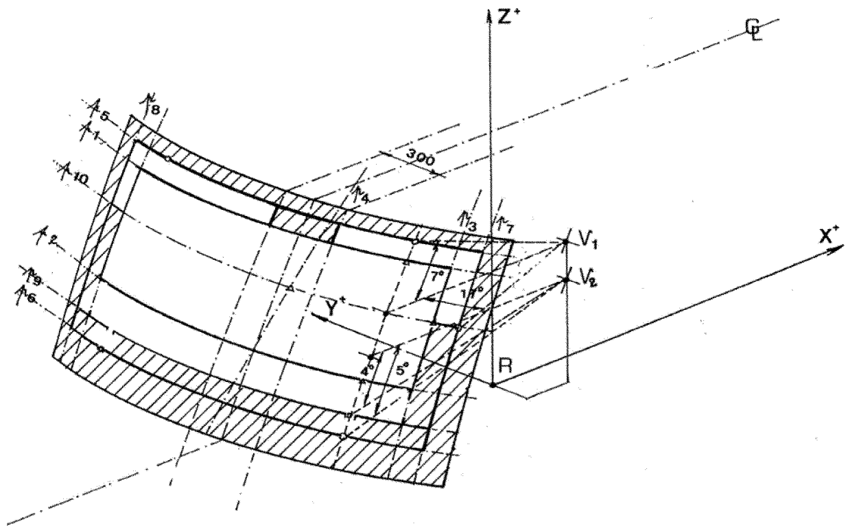
Figure 19(a): Reduced test area "B" Upper obscuration area as defined in paragraph S6.15.3.2.4.2.2.
